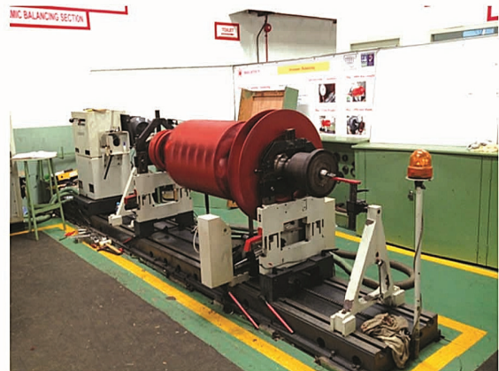
Balancing of Motor
